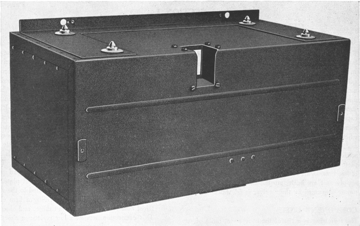
FIGURE 2—BOTTOM AND BACK VIEW OF CABINET RADIO RECEIVER BC-348-H
