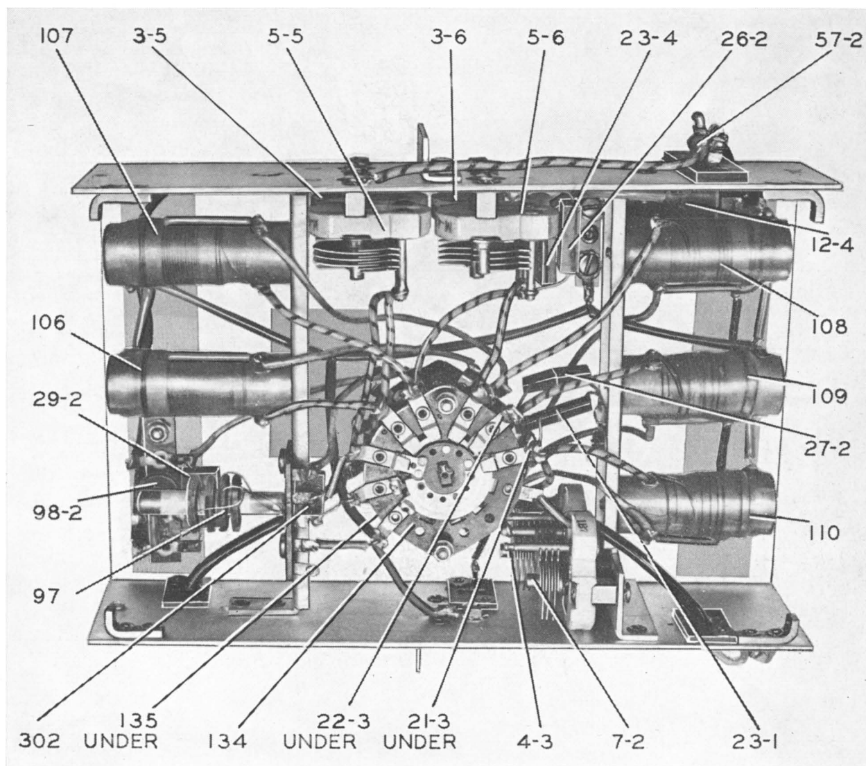
FIGURE 19—DETECTOR UNIT
