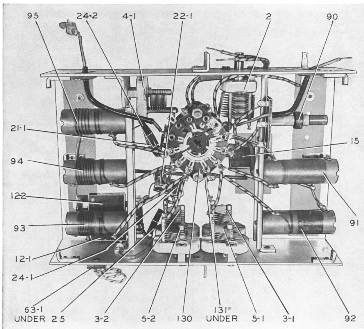
FIGURE 17—ANTENNA UNIT
