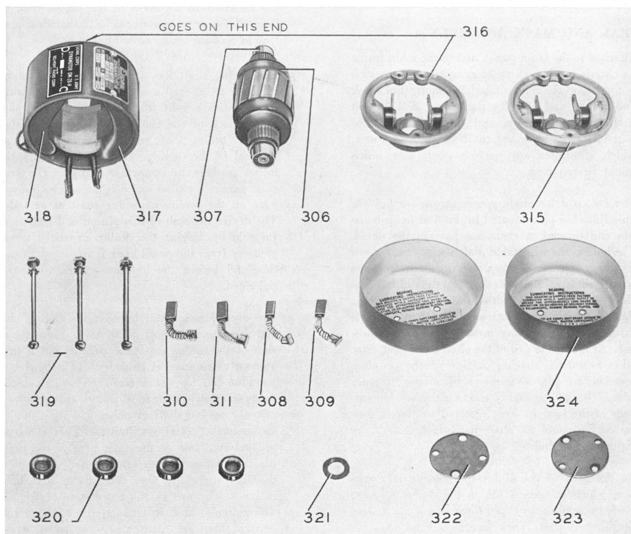
FIGURE 13—DYNAMOTOR DM-28-H, DISASSEMBLED
