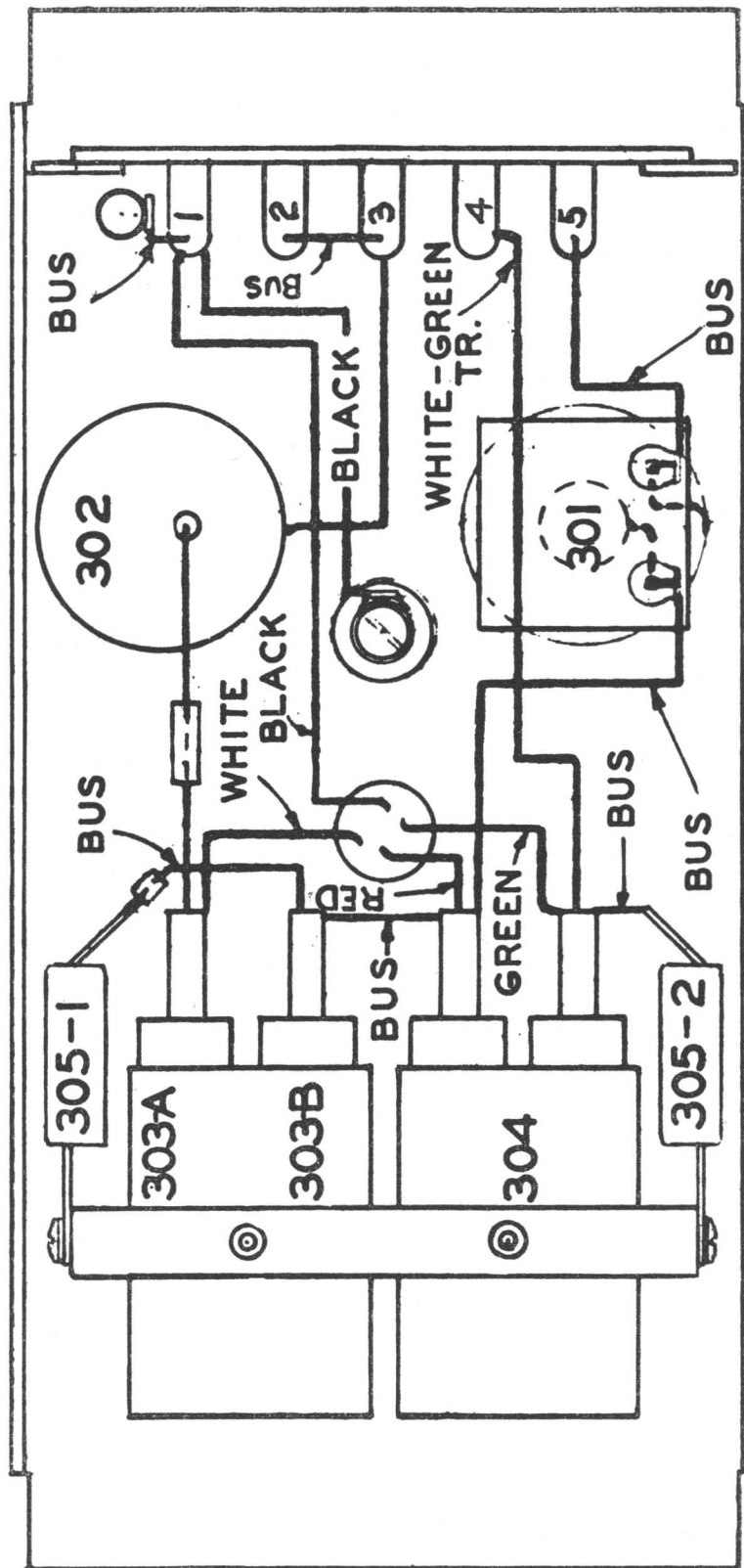
FIGURE 34—RADIO RECEIVER BC-348-H: WIRING DIAGRAM, DYNAMOTOR ASSEMBLY
