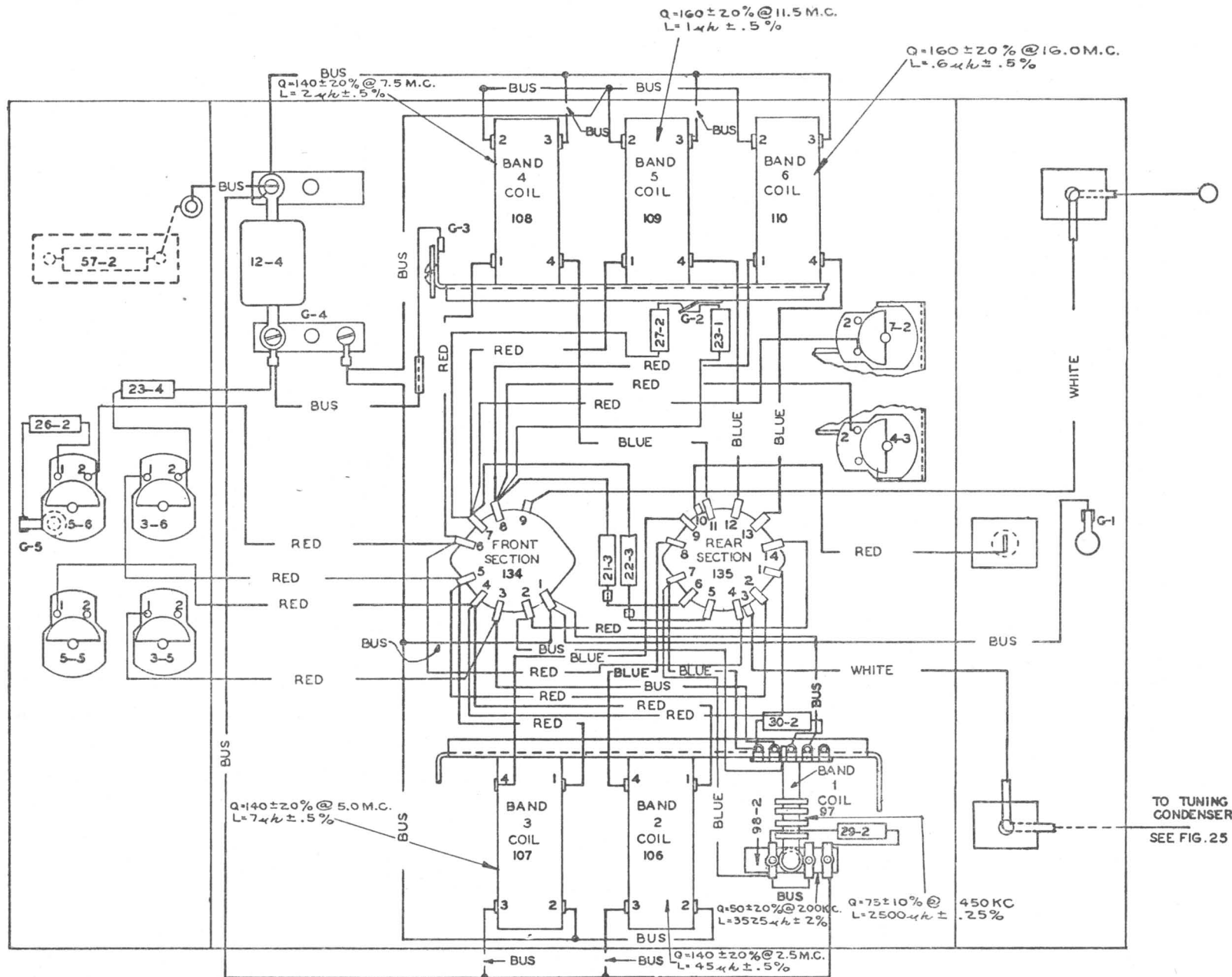
FIGURE 28—RADIO RECEIVER BC-348-H: WIRING DIAGRAM, DETECTOR UNIT
