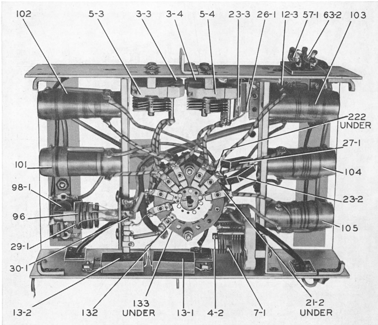
FIGURE 18—R-F UNIT
