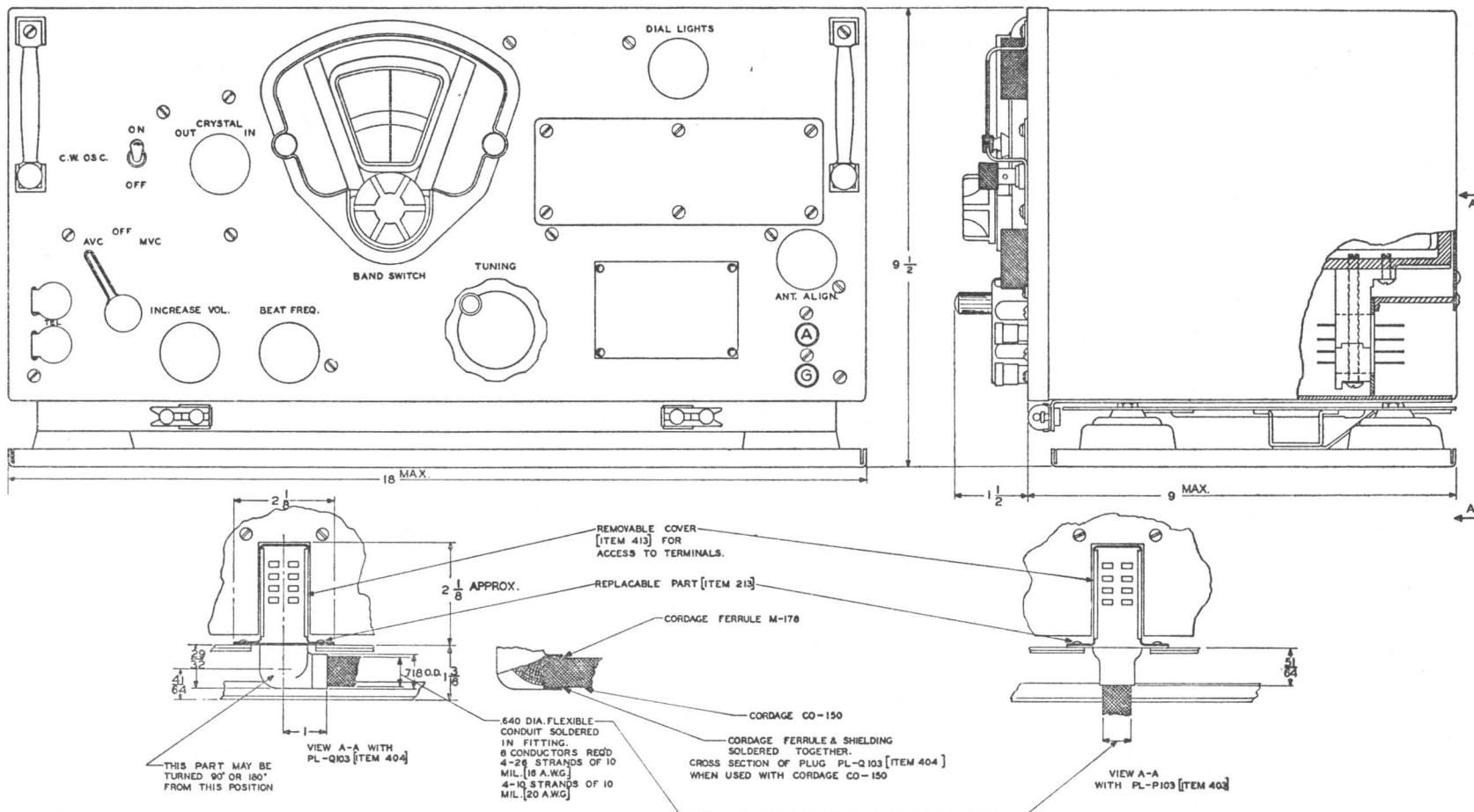
FIGURE 37—Radio Receiver BC-348-H: OUTLINE DIMENSIONAL DRAWING
