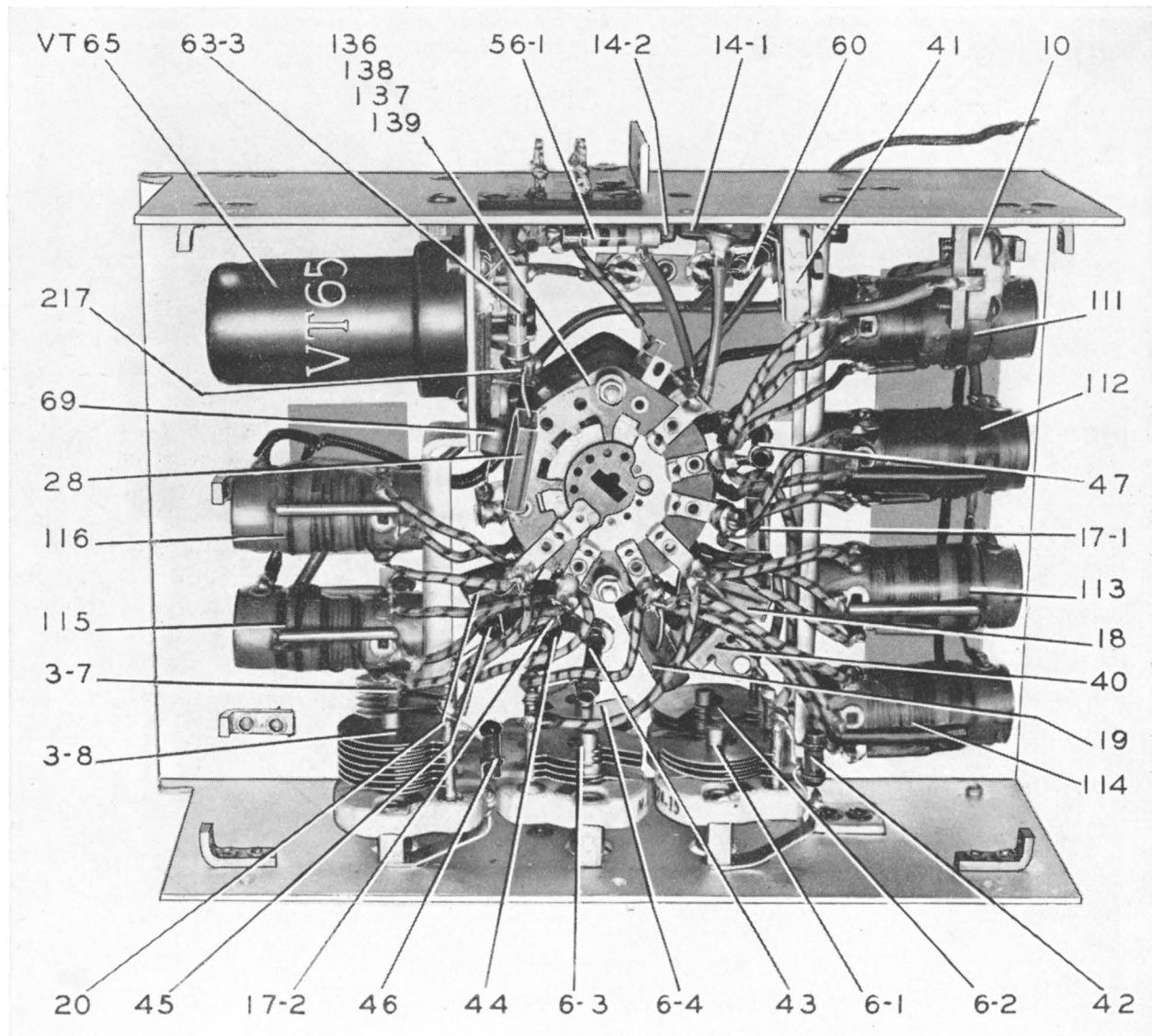
FIGURE 20—OSCILLATOR UNIT
