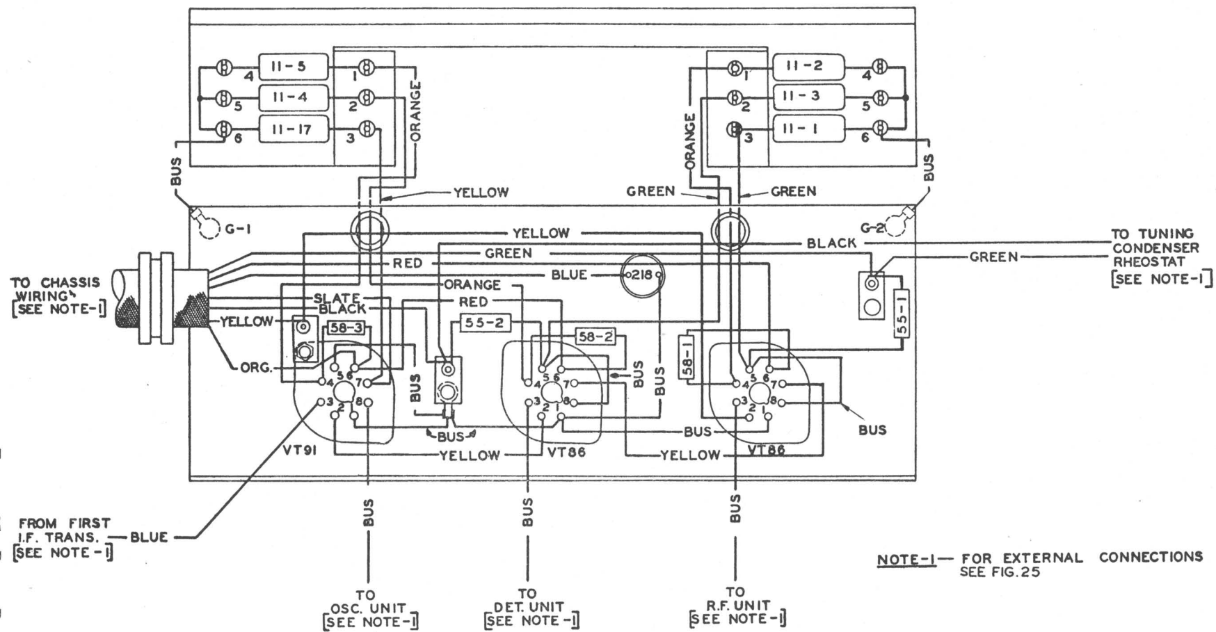
FIGURE 25—RADIO RECEIVER BC-348-H: WIRING DIAGRAM, TUBE SHELF
