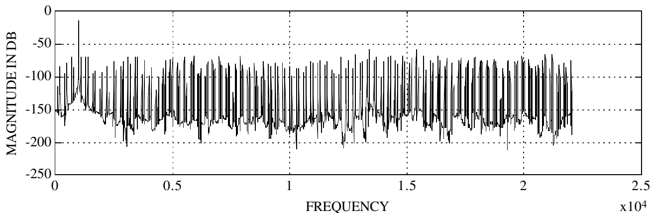
Figure 5: Error spectrum after downsampling from 96 kHz to 44.1 kHz
