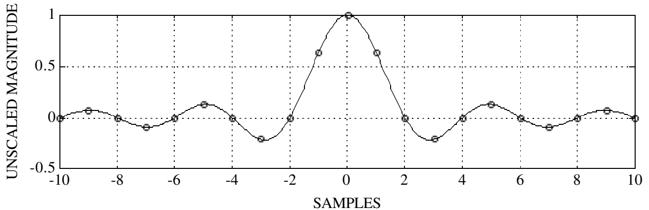
Figure 3: Possible Downsampling Filter from 96 kHz to 48 kHz
