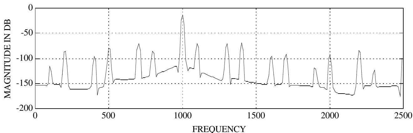
Figure 6: Error spectrum after downsampling from 96 kHz to 44.1 kHz
