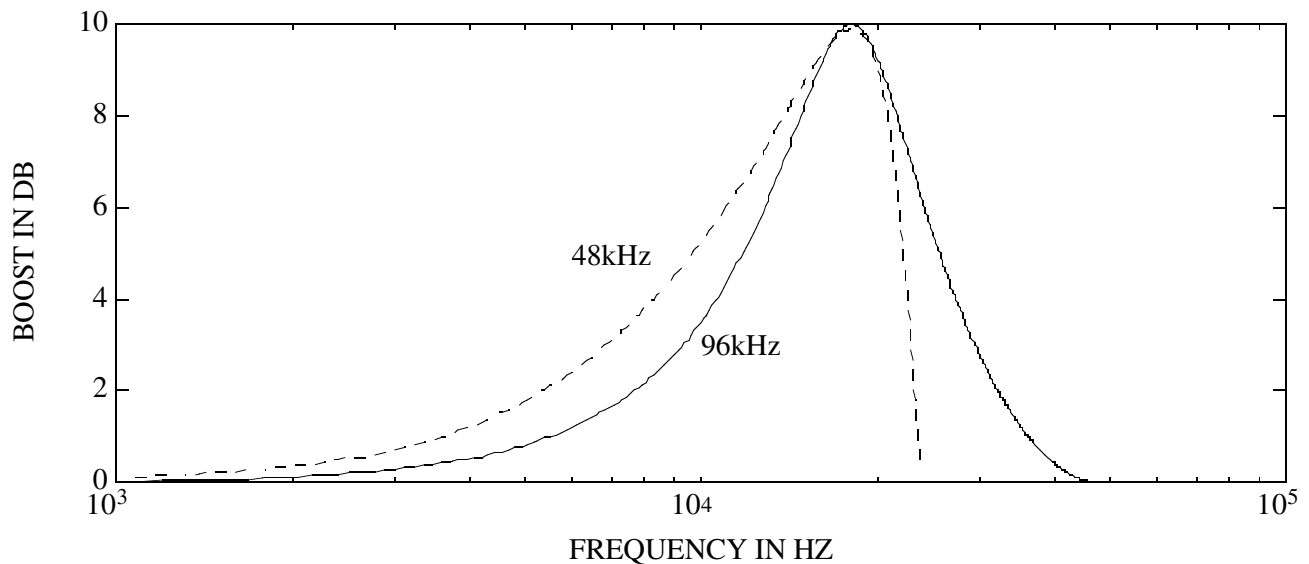
Figure 2: 18kHz presence filter at 48 kHz and 96 kHz sampling rates
