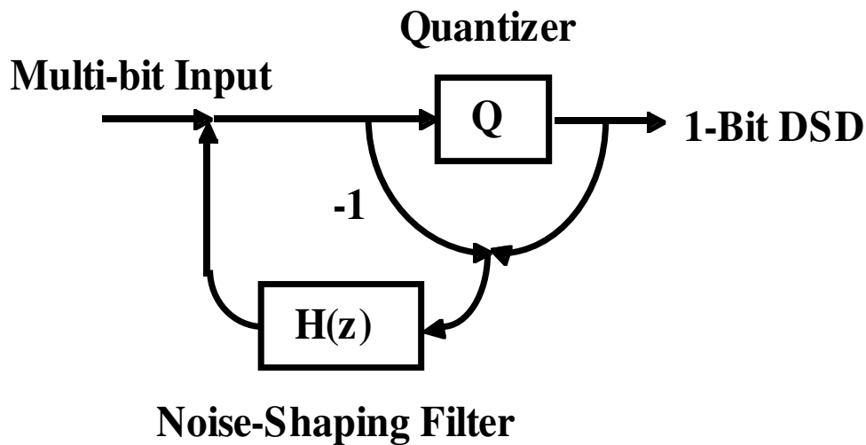
Figure 7: Quantizer with Noise Shaper
