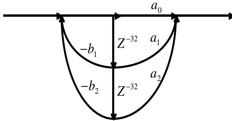
Figure 8: Possible second-order digital filter for DSD
