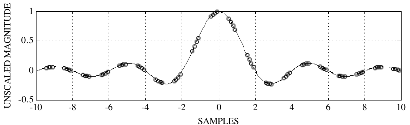
Figure 4: Possible Downsampling Filter from 96 kHz to 44.1 kHz
