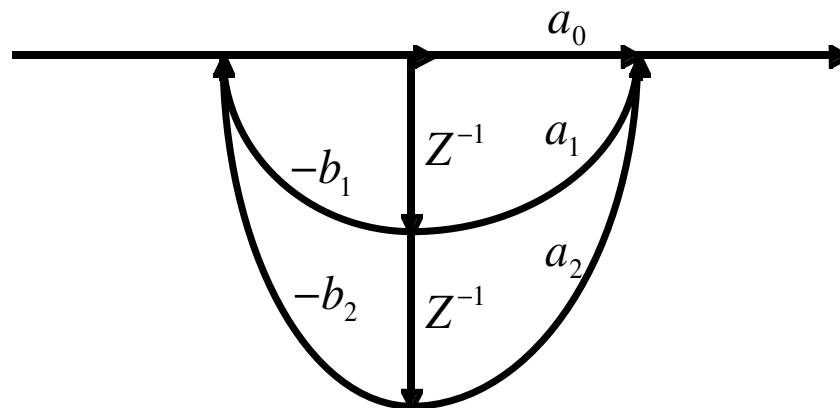
Figure 1: One form of a second-order digital filter
