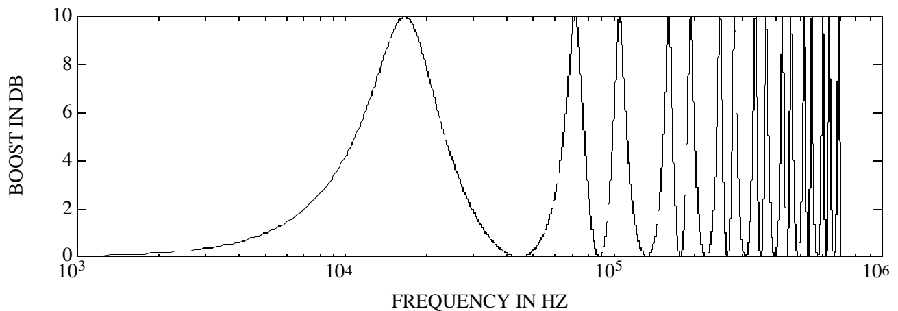
Figure 9: Response of 18 kHz Presence Filter with 32-sample Delays
