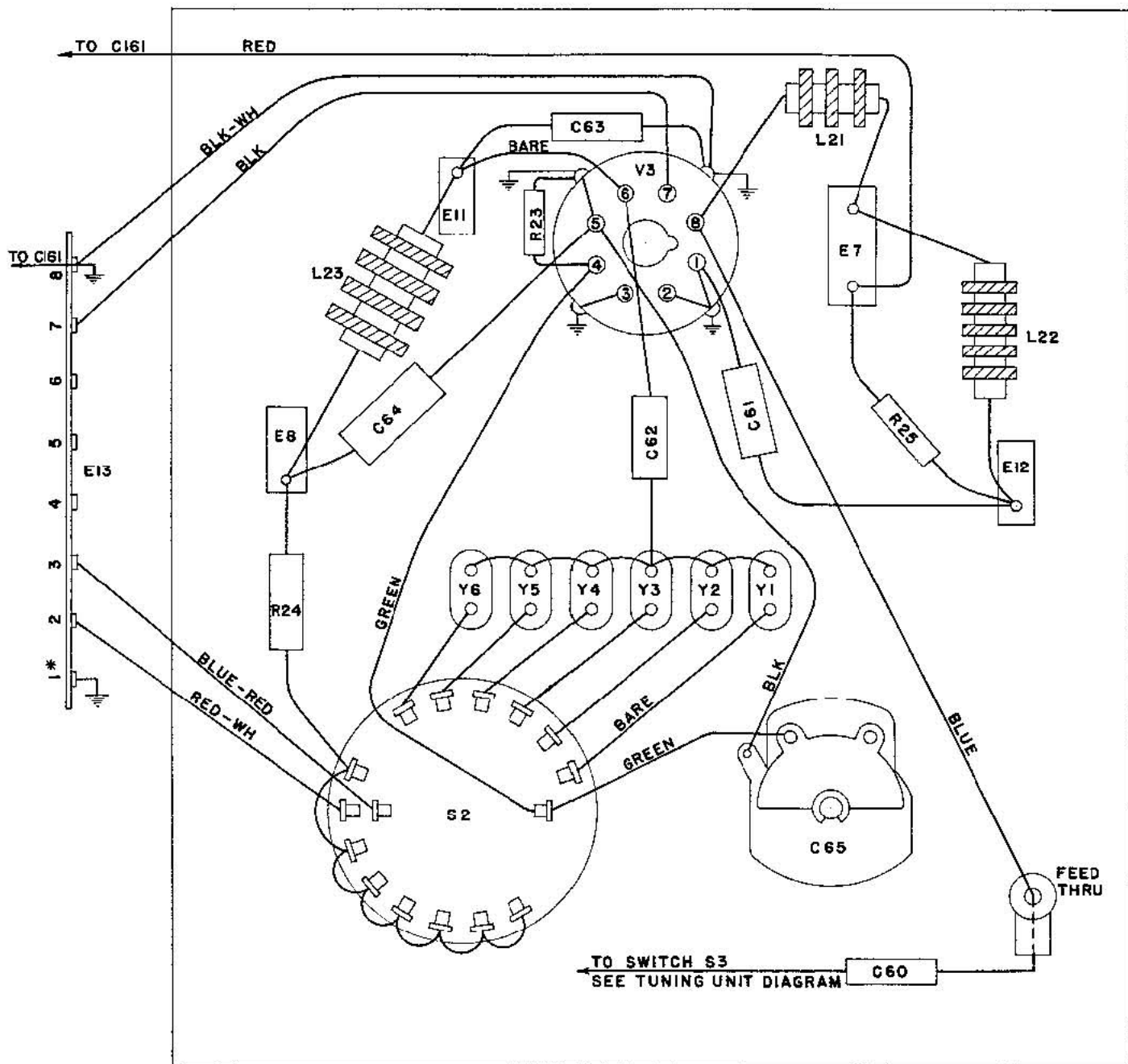
FIGURE 14 CONNECTION DIAGRAM FREQUENCY CONTROL UNIT
