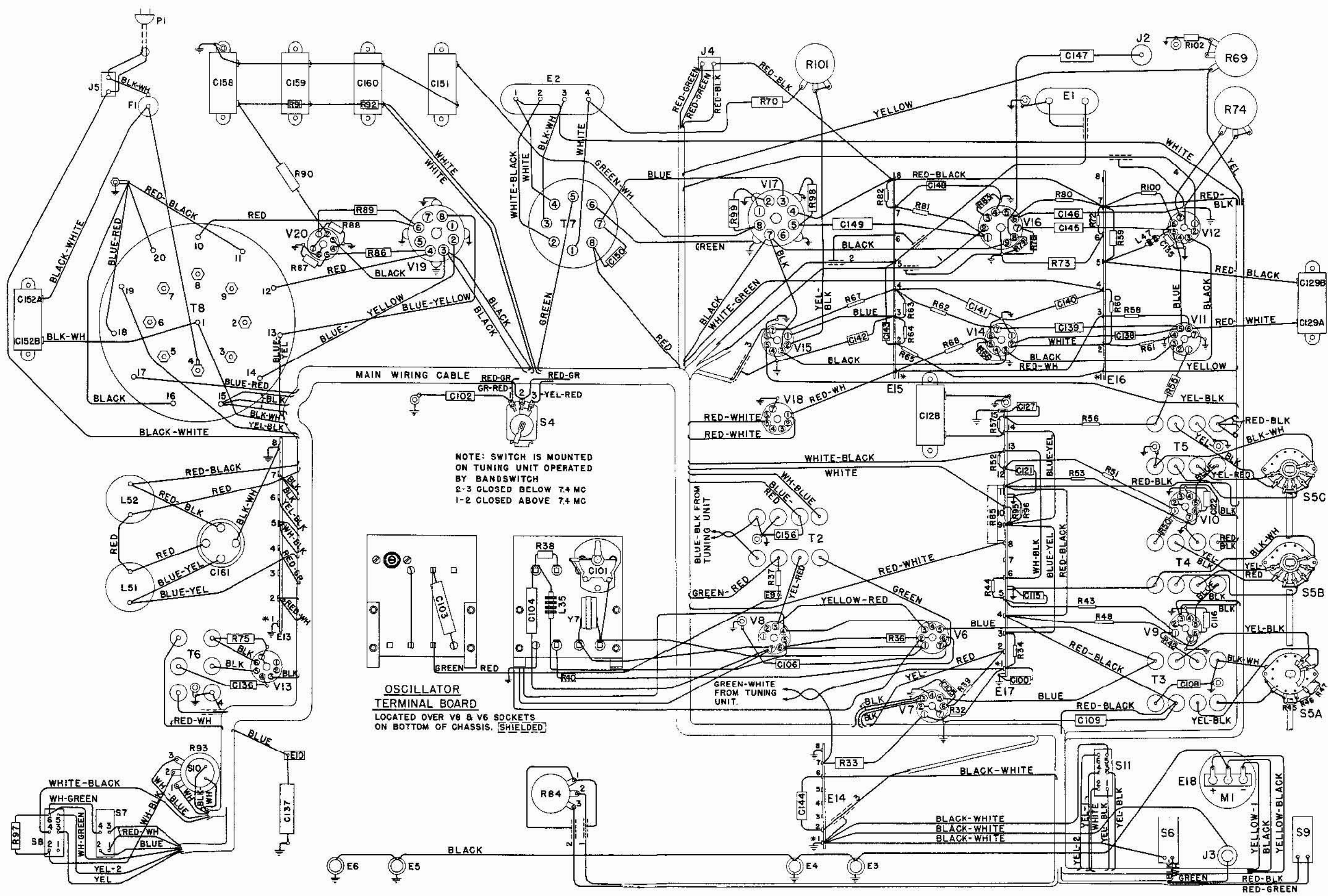
FIGURE NUMBER 12 CONNECTION DIAGRAM-RECEIVER CHASSIS
