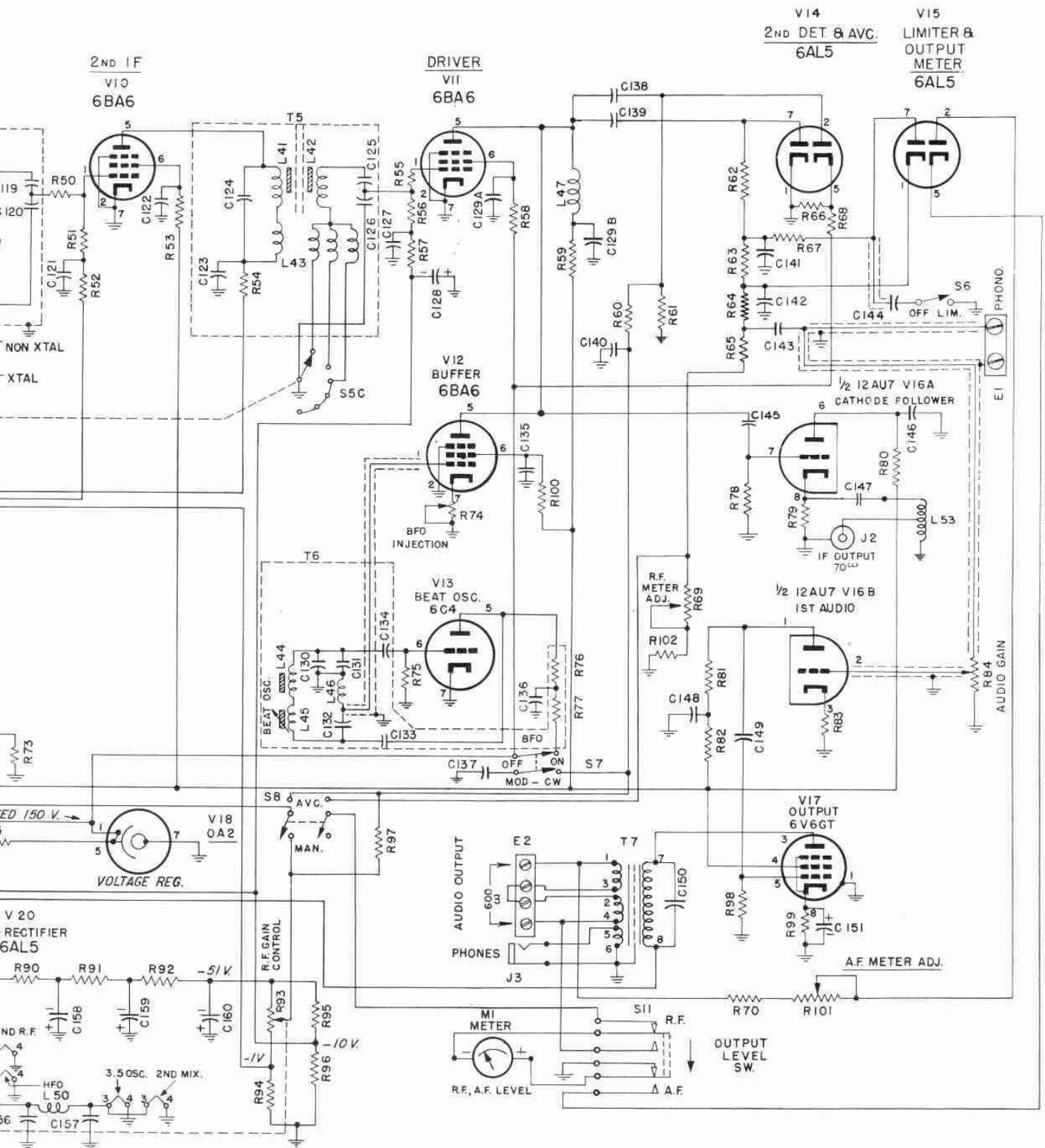
FIG. 11 CIRCUIT DIAGRAM OF RECEIVER
