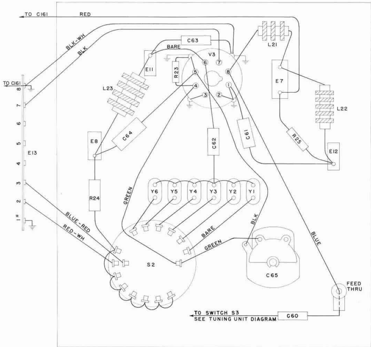
FIGURE 14 CONNECTION DIAGRAM FREQUENCY CONTROL UNIT
