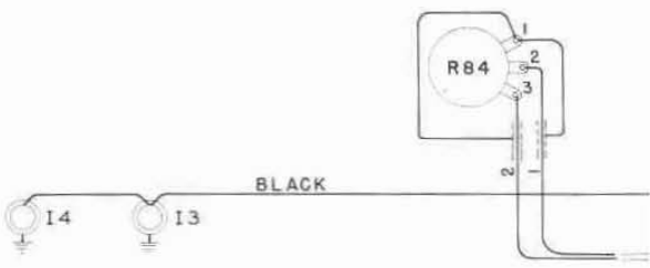
OSCILLATOR TERMINAL BOARD LOCATED OVER V8 & V6 SOCKETS ON BOTTOM OF CHASSIS. [SHIELDED]
