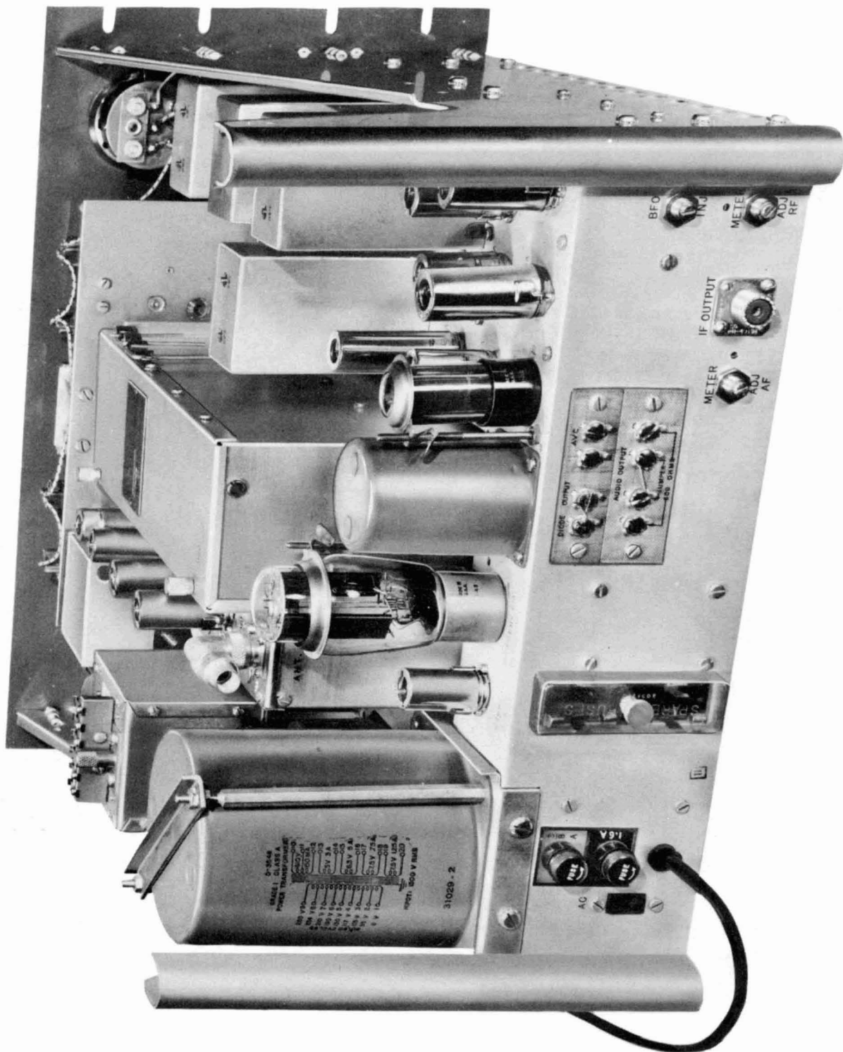
FIG. 6 REAR VIEW OF RECEIVER
