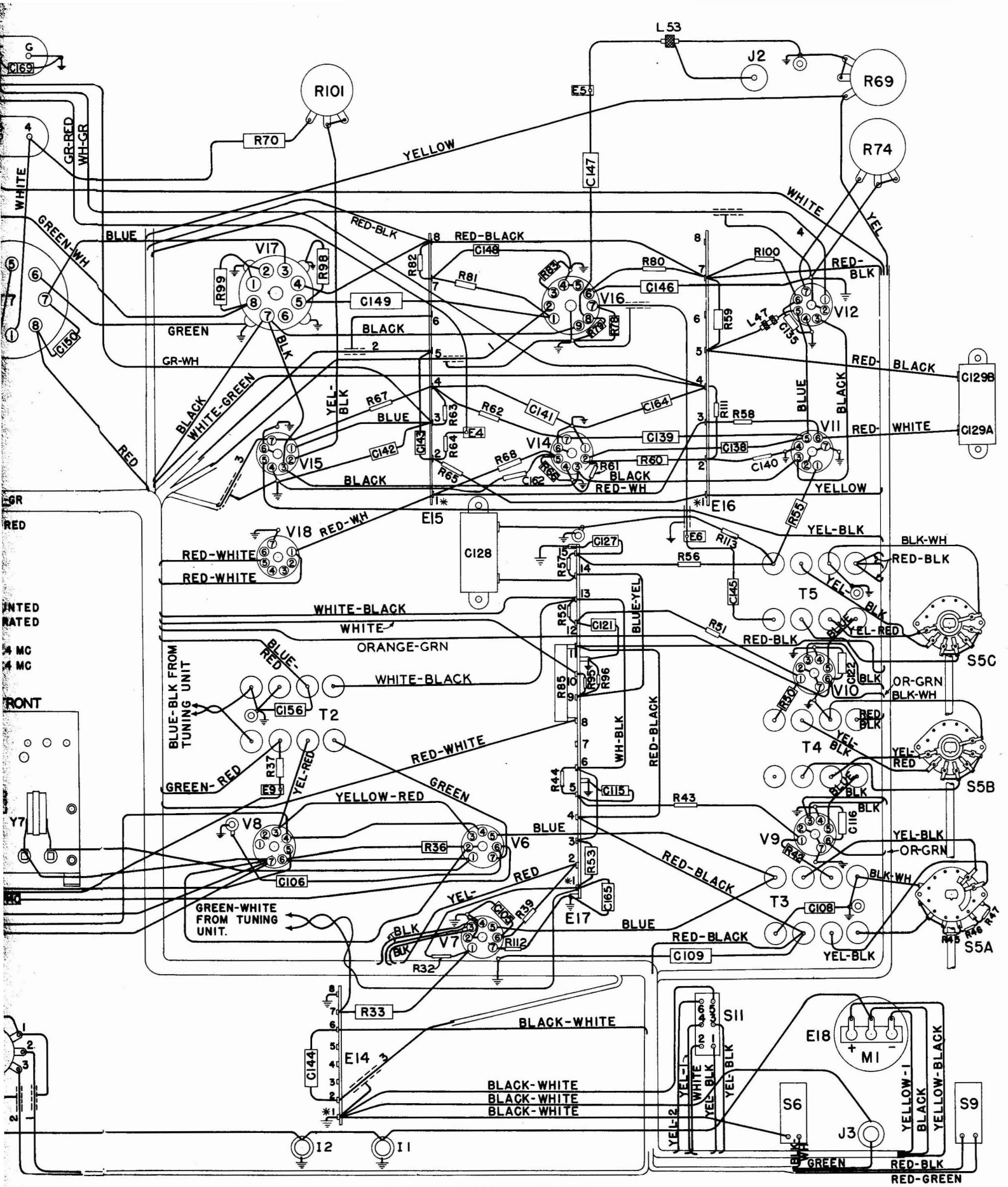
FIGURE NUMBER 14 CONNECTION DIAGRAM-RECEIVER CHASSIS
