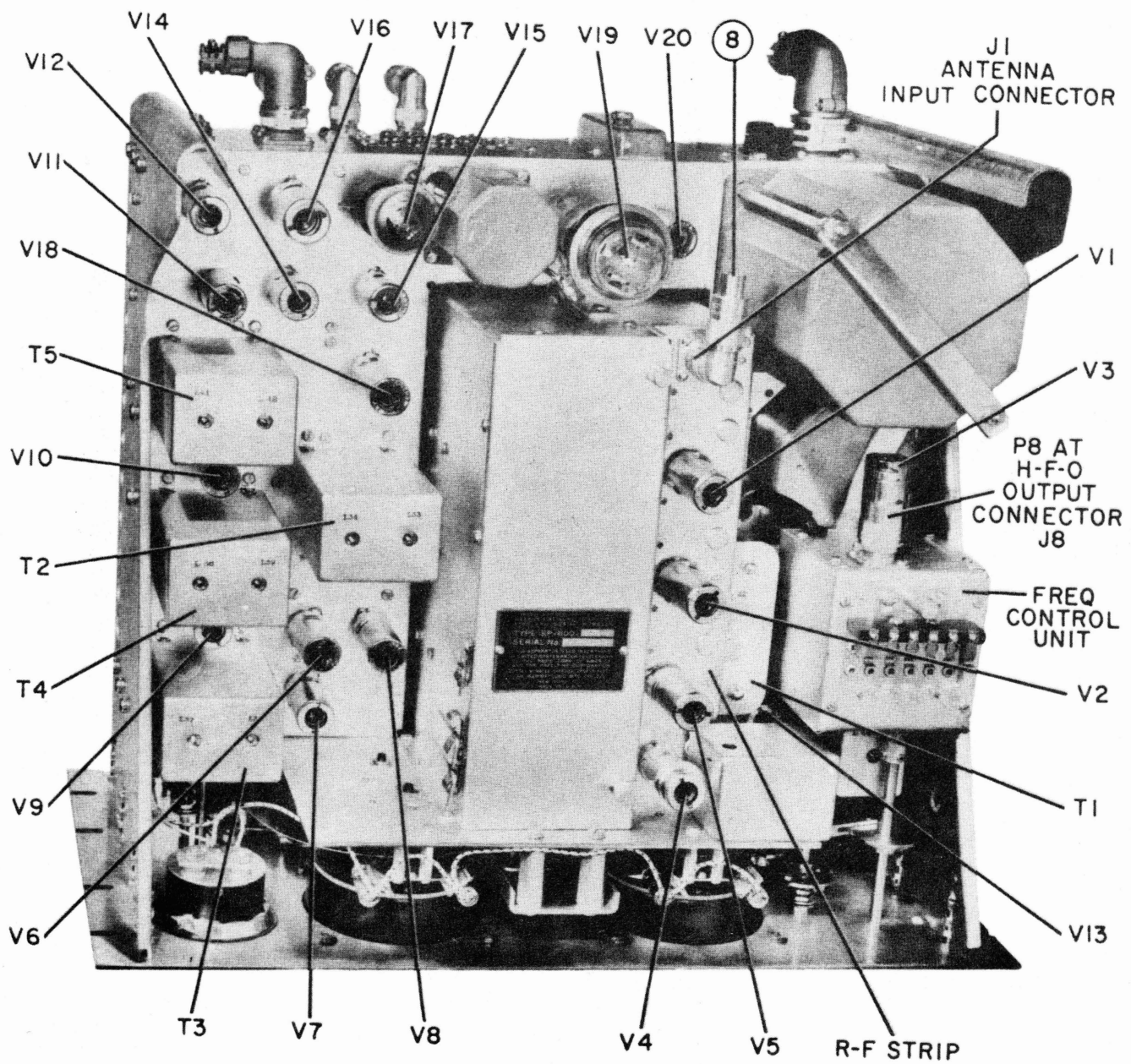
Figure 7. Radio Receiver, Top View of Chassis
