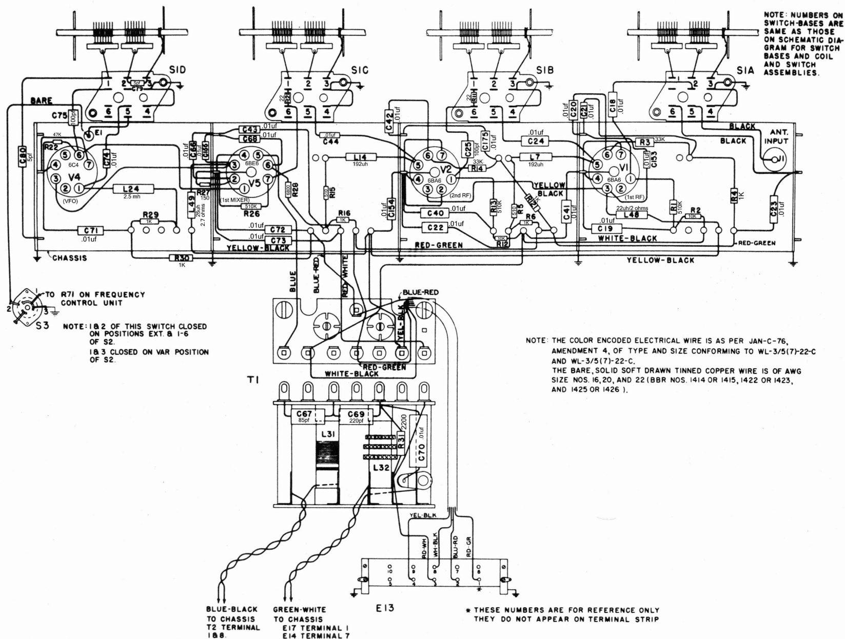
Figure 11. Radio Receiver, Tuning Unit Connection Diagram
